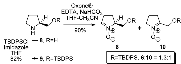
Scheme 2. Preparation of Nitron 6 from L-Prolinol
