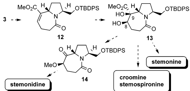
Scheme 4. Synthetic Plan from 3 to the Target Alkaloids
