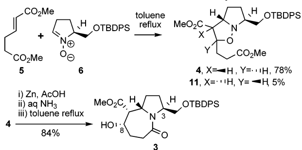
Scheme 3. Construction of the Azabicyclic Core
