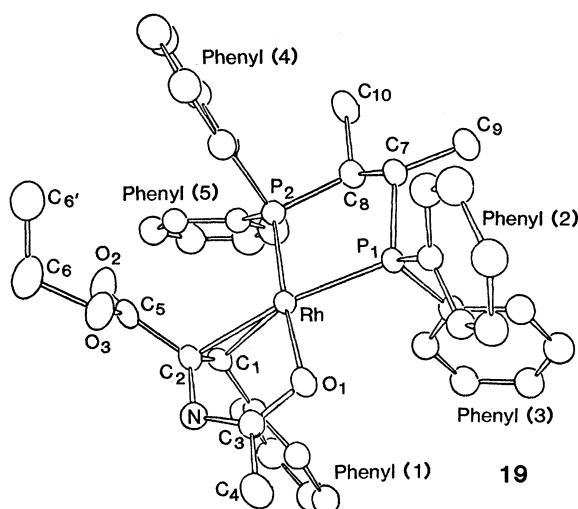
Fig. 3. Structure of the predominant diastereomer of [\text{Rh}(\text{S,S-CHIRAPHOS})(\text{EAC})]^+ .
