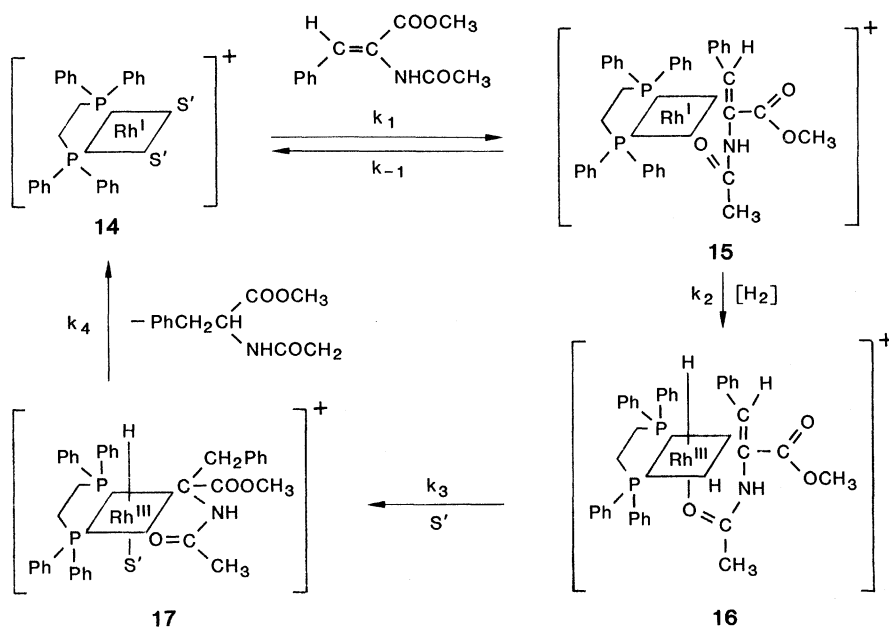
Fig. 1. Mechanism of the [\text{Rh}(\text{DIPHOS})]^+ -catalyzed hydrogenation of methyl-( Z )- \alpha -acetamidocinnamate (MAC).
