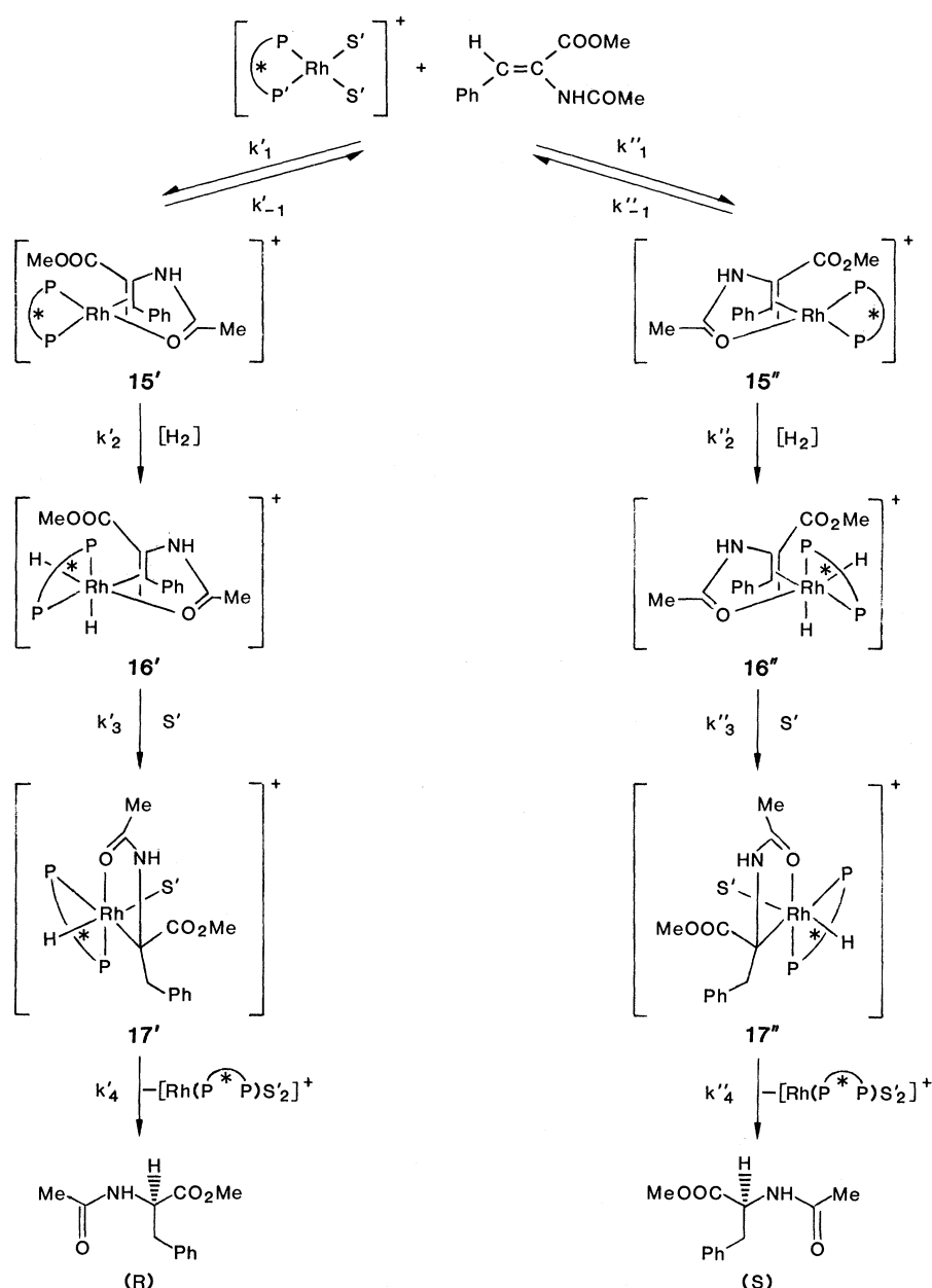
Fig. 2. Mechanistic scheme for the hydrogenation of a prochiral substrate (MAC) with a catalyst containing a chiral chelating diphosphine ligand ( P^*P , CHIRAPHOS or DIPAMP; S' , methanol).
